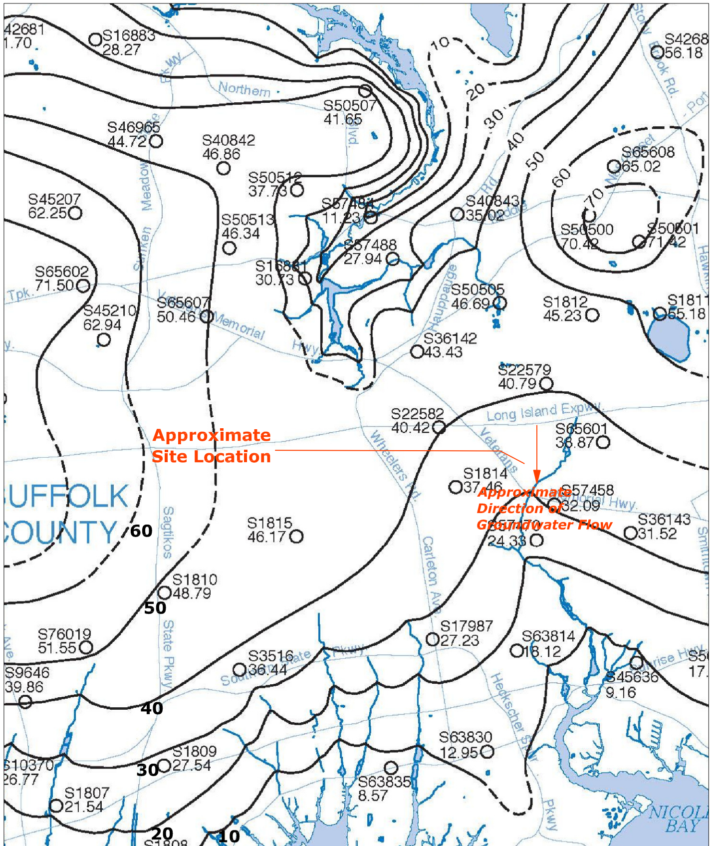
FIGURE 2-2 WATER TABLE CONTOUR MAP
